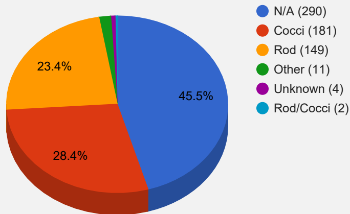
Bacteria samples by morphology(637 Samples)
