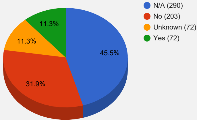
Bacteria samples by spore-forming(637 Samples)
