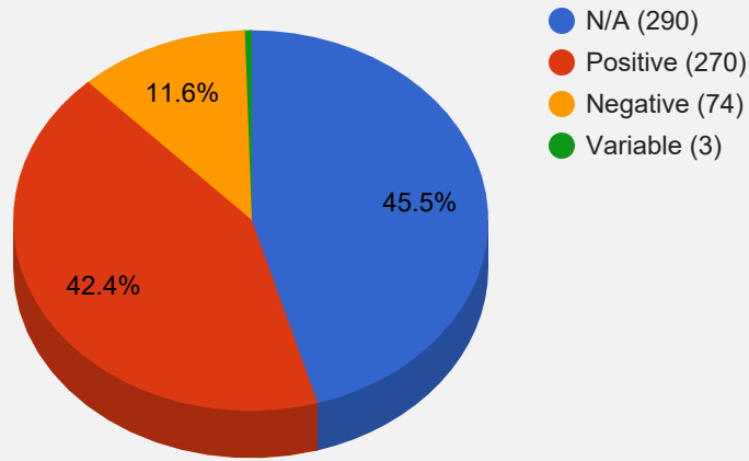
Bacteria samples by gram reaction(637 Samples)
